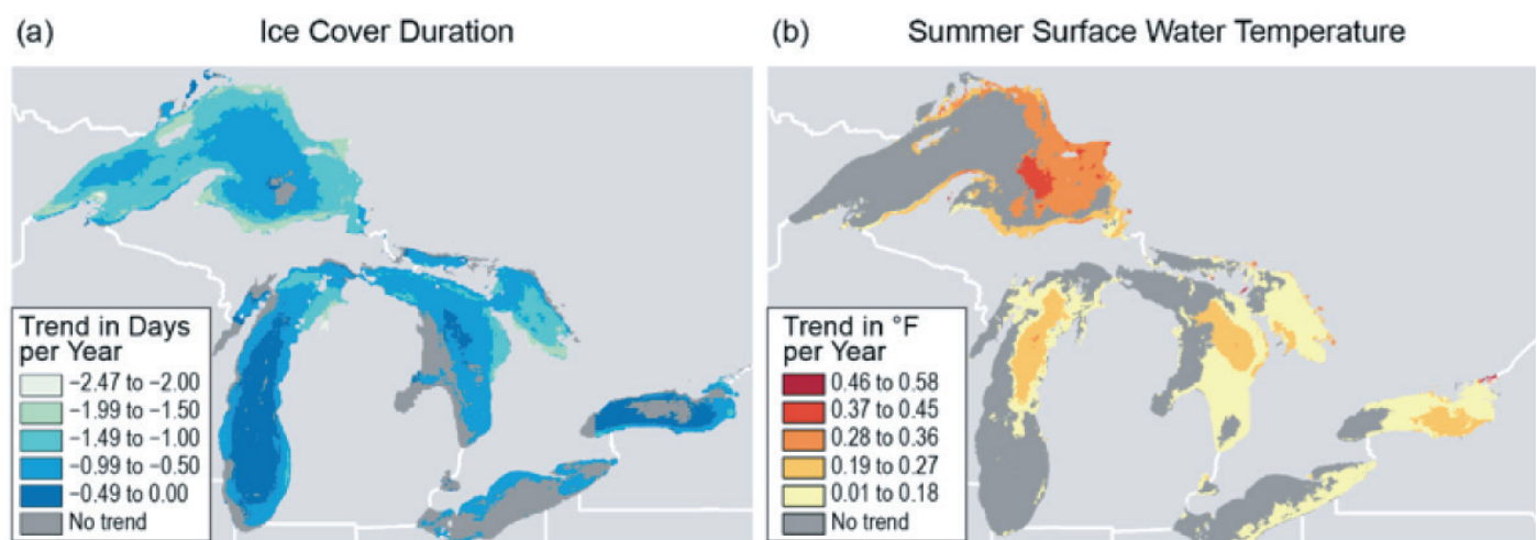
Figure 5: Change in summer temperatures in the Great Lakes from 1994 to 2013
