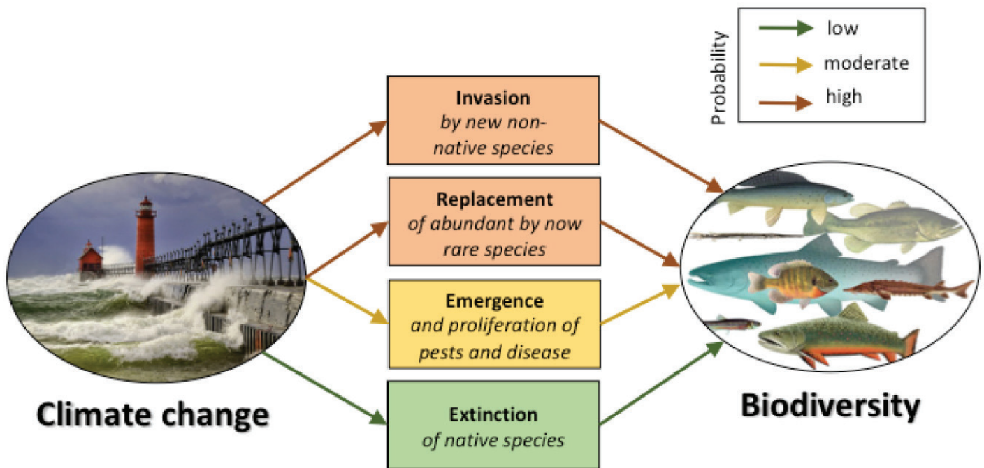
Figure 8: The impact of Climate Change on biodiversity in the Great Lakes
