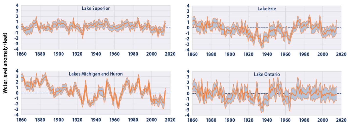
Figure 7: Water levels of the Great Lakes
