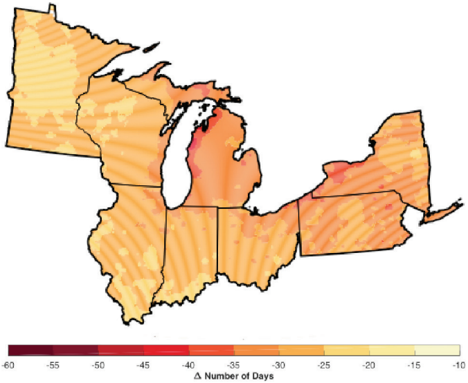
Figure A4. Change in the number of days with temperature less than 32°F for U.S. states bordering the Great Lakes from the (a) higher (RCP8.5) and (b) lower (RCP4.5) scenarios for the 2085 (2070-2099) time period relative to 1976-2005. (Figure source: NOAA/NCEI)
