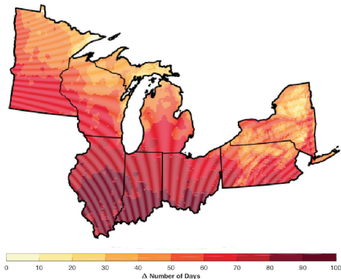
Figure A3. Change in the number of days with temperature greater than 90°F for U.S. states bordering the Great Lakes from the (a) higher (RCP8.5) and (b) lower (RCP4.5) scenarios for the 2085 (2070-2099) time period relative to 1976-2005. (Figure source: NOAA/NCEI)
