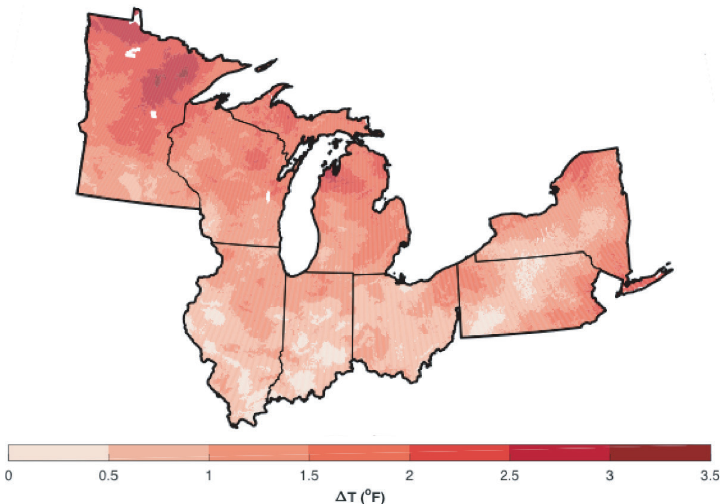
Figure 3: Annual temperature difference: nClimDiv (1986 – 2016) – (1901 – 1960)
