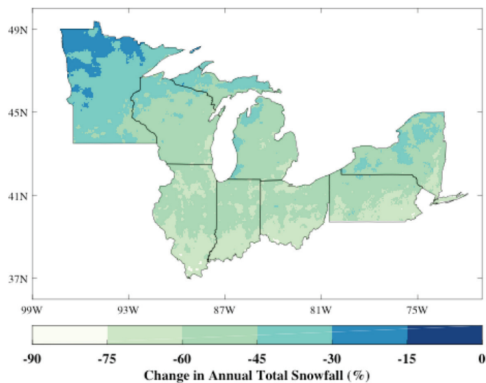
Figure A6: Change in annual total snowfall between 1984-2013 and 1954-1983
