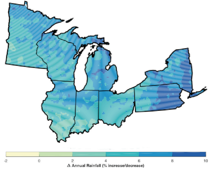
Figure A2. Change in annual precipitation (as equivalent rainfall) (%) for U.S. states bordering the Great Lakes from the (a) higher (RCP8.5) and (b) lower (RCP4.5) scenarios for the 2085 (2070-2099) time period relative to 1976-2005. (Figure source: NOAA/NCEI)
