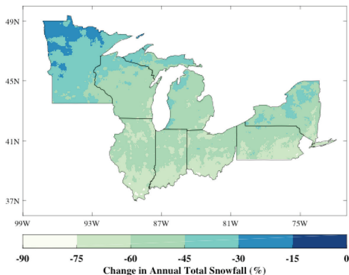
(a) Change in annual total snowfall from RCP8.5 (1976-2005 and 2071-2100)
