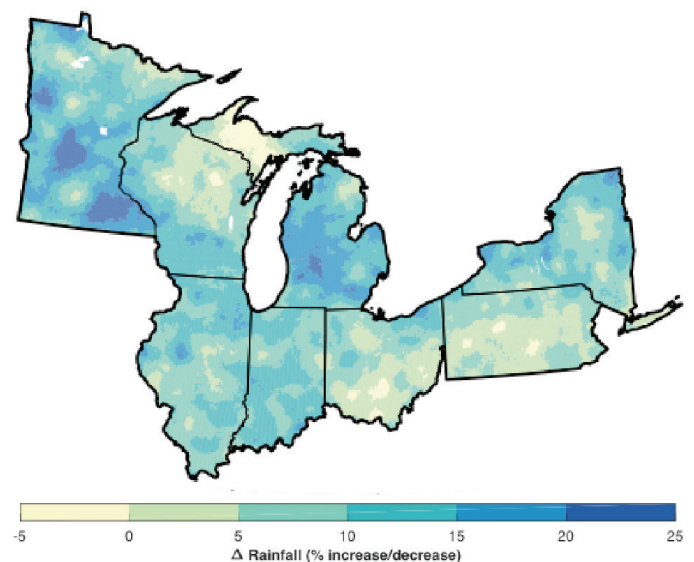
Figure A1: Change in average annual rainfall: nClimDiv (1986 - 2016) - (1901 - 1960)
