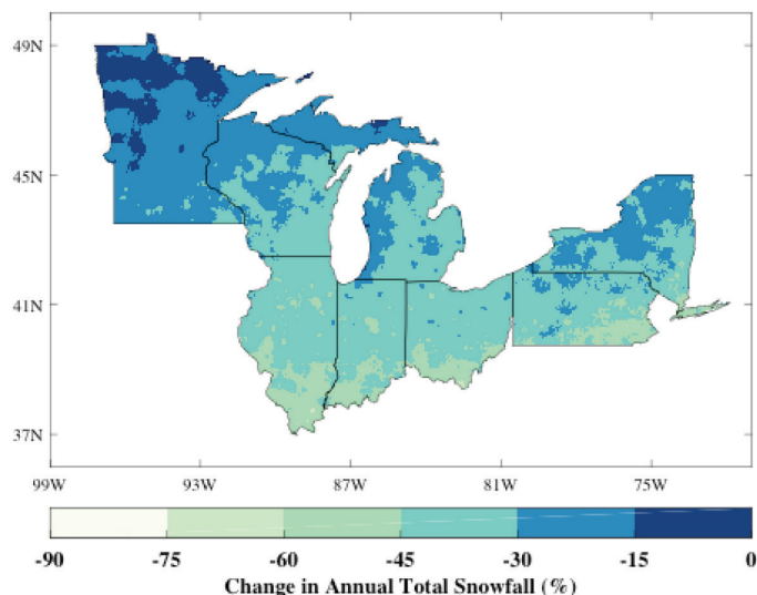
(b) Change in annual total snowfall from RCP4.5 (1976-2005 and 2071-2100)
