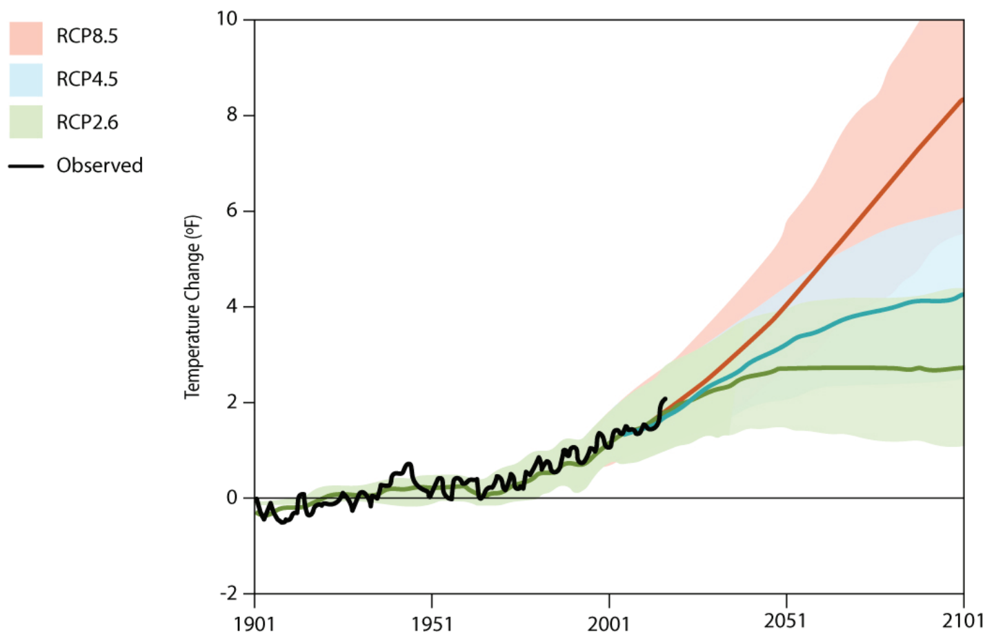
Figure 2: Projected Global Temperatures
