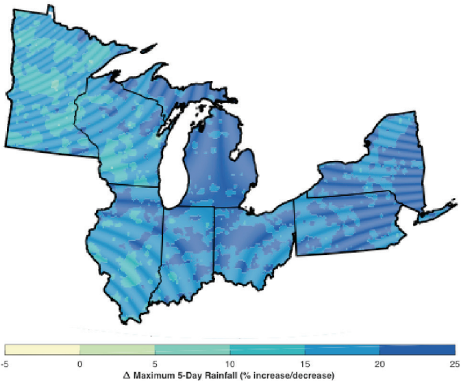
Figure A5. Percentage change in annual maximum five-day rainfall amounts for U.S. states bordering the Great Lakes from the (a) higher (RCP8.5) and (b) lower (RCP4.5) scenarios for the 2085 (2070-2099) time period relative to 1976-2005. (Figure source: NOAA/NCEI)
