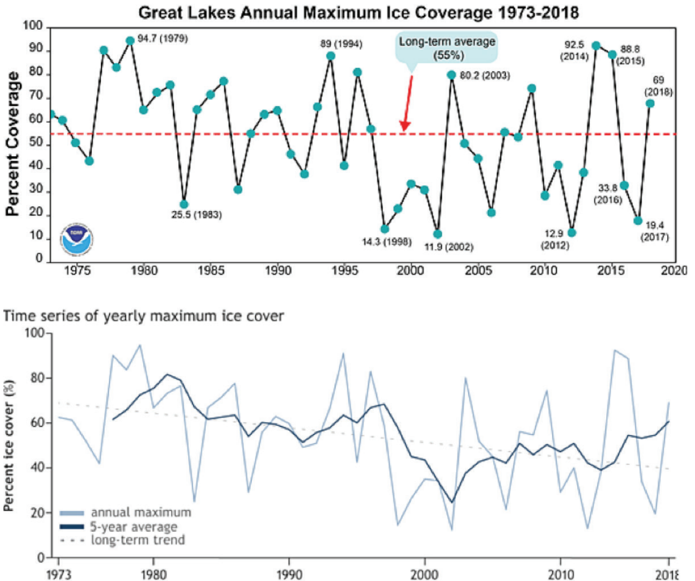
Figure 6: Great Lakes ice coverage
