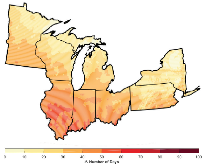
Figure A3. Change in the number of days with temperature greater than 90°F for U.S. states bordering the Great Lakes from the (a) higher (RCP8.5) and (b) lower (RCP4.5) scenarios for the 2085 (2070-2099) time period relative to 1976-2005. (Figure source: NOAA/NCEI)
