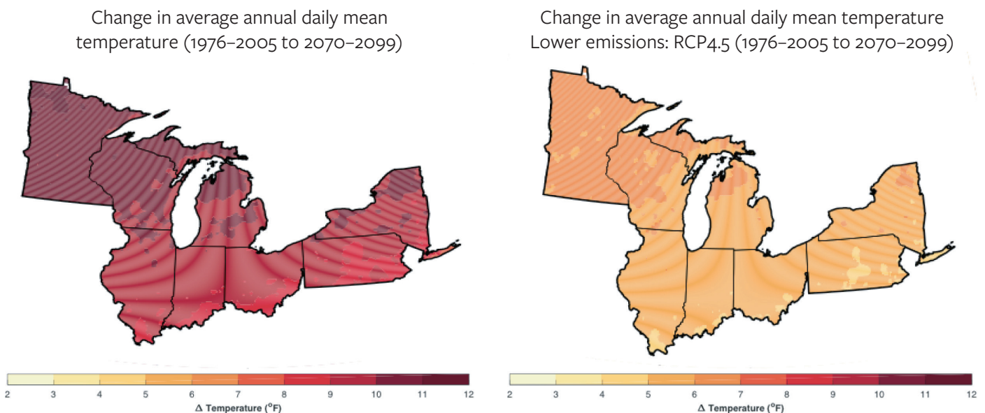
Figure 4: Projected change in annually average temperature (°F) for U.S. states bordering the Great Lakes
